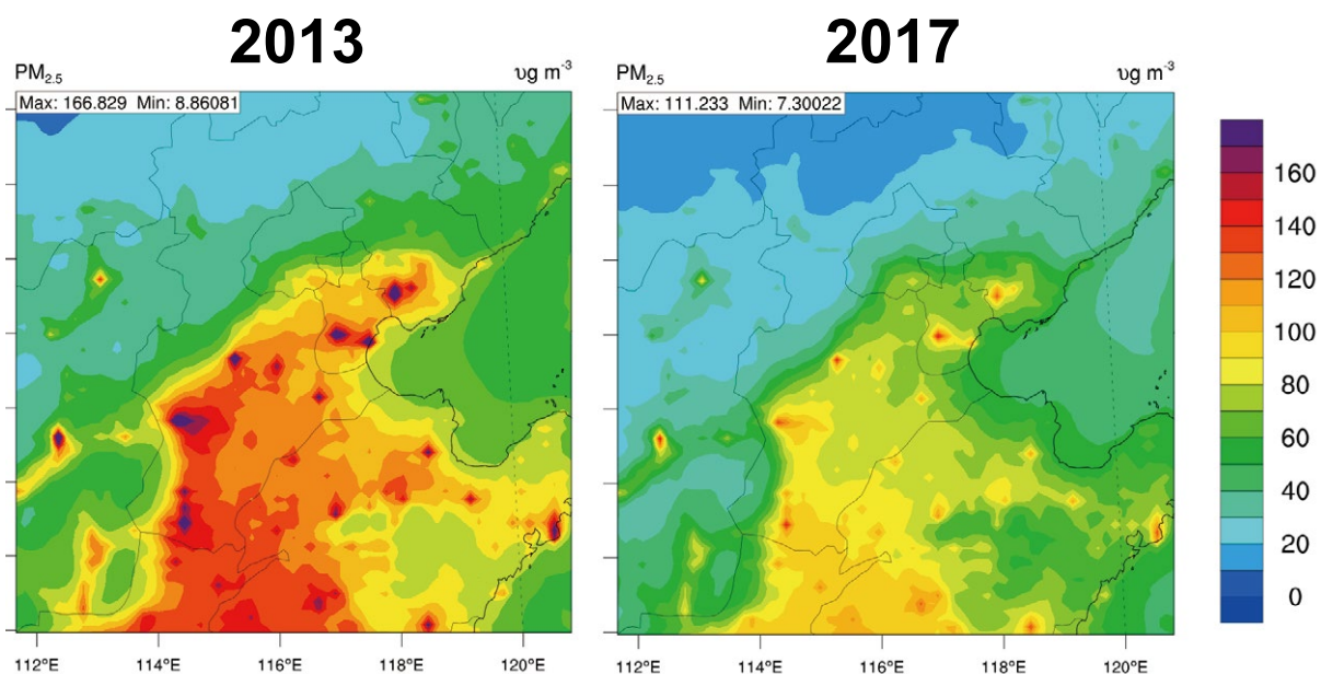
Figure11 Spatial distribution of annual average PM_{2.5} concentrations in Beijing-Tianjin-Hebei and Surrounding Areas (2013, 2017)
