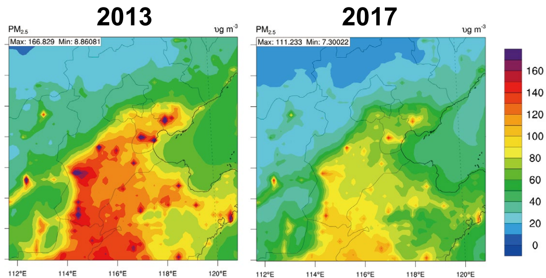
Figure 6.5 Spatial distributions of annual average \text{PM}_{2.5} concentrations in Beijing and its surrounding areas (2013, 2017)
