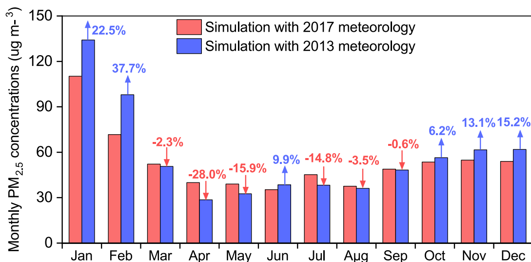
Figure 6.4 Monthly simulation of \text{PM}_{2.5} concentration in Beijing under 2013 and 2017 meteorological conditions at 2017 emission levels
