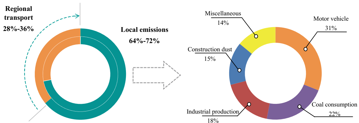
Figure 2.3 PM 2.5 source apportionment results for Beijing, 2013
